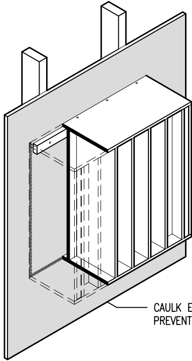
SECTIONAL ISOMETRIC VIEW SHOWING CLEAT LOCATION
