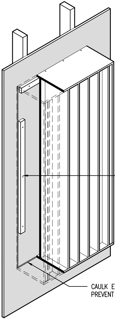
SECTIONAL ISOMETRIC VIEW SHOWING CLEAT LOCATION
