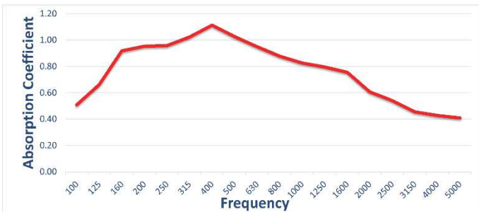
The sound absorption chart above represents the Perfect® Micro Panel wall or ceiling mounted on 2" wood firrings with 2" 6lb/ft 3 fiberglass board installed between each furring. Other data can be provided upon request.
