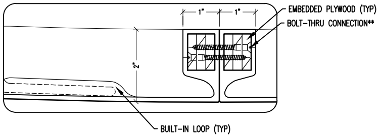
JOINING DETAIL (SECTION)
