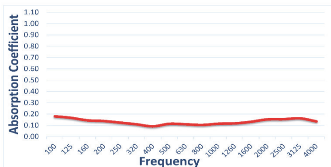
The sound absorption chart above represents the Waveform® Monoradial direct wall or ceiling mounted. Other data can be provided upon request.
