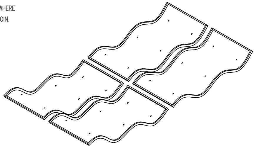
SPLINE ARRAY (EXPLODED)
