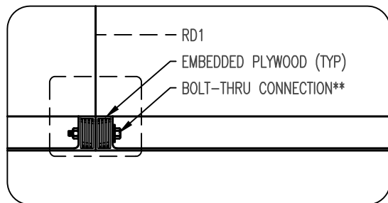
JOINING DETAIL (SECTION)
