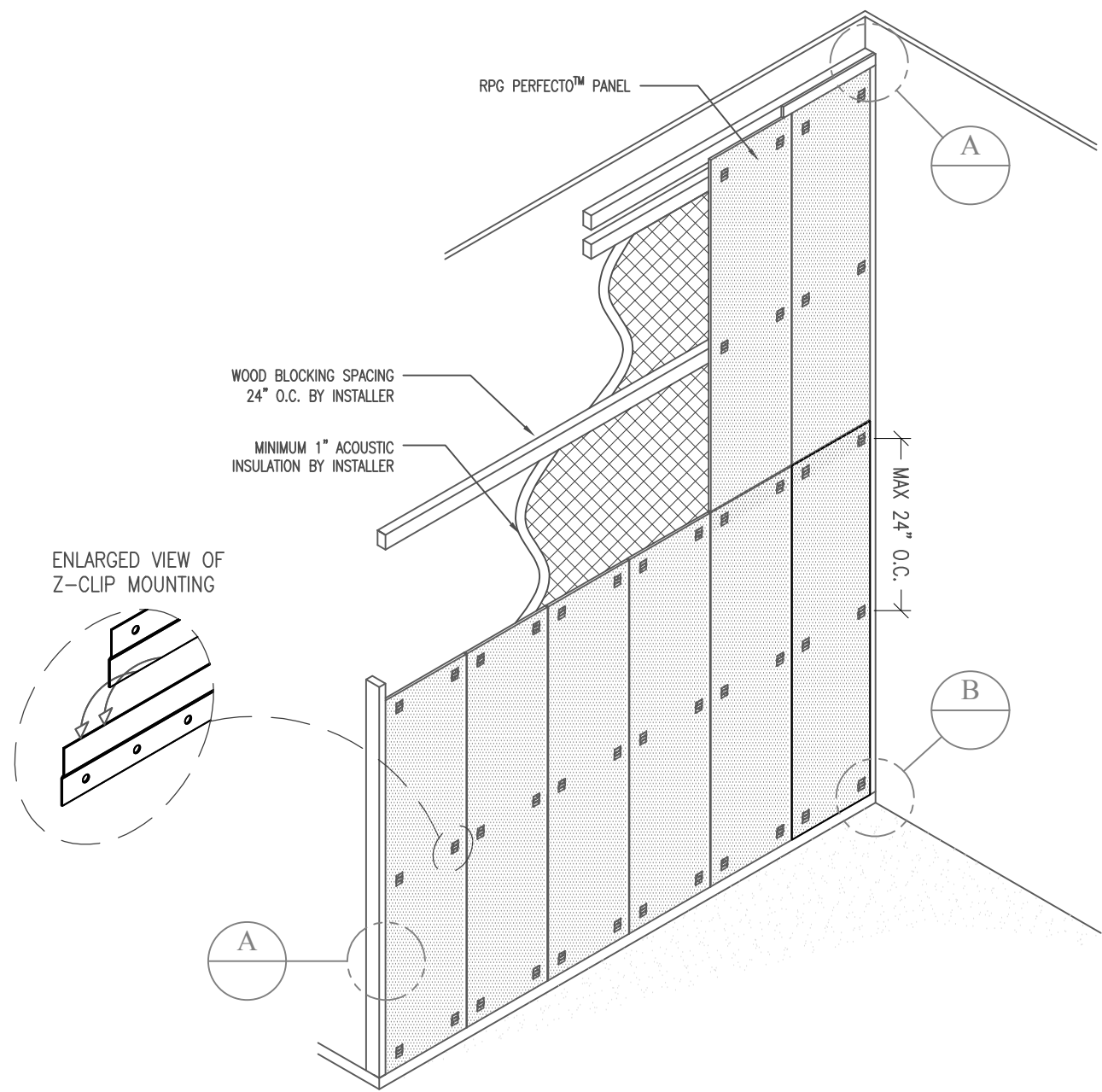
ISOMETRIC VIEW (NTS)
