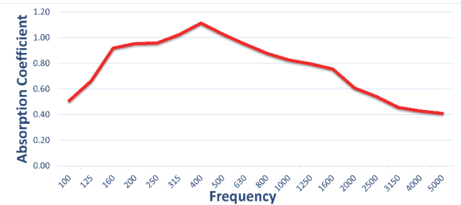
The sound absorption chart above represents the Perfect® Micro Plank wall or ceiling mounted on 2" wood firrings with 2" 6lb/ft 3 fiberglass board installed between each furring. Other data can be provided upon request.
