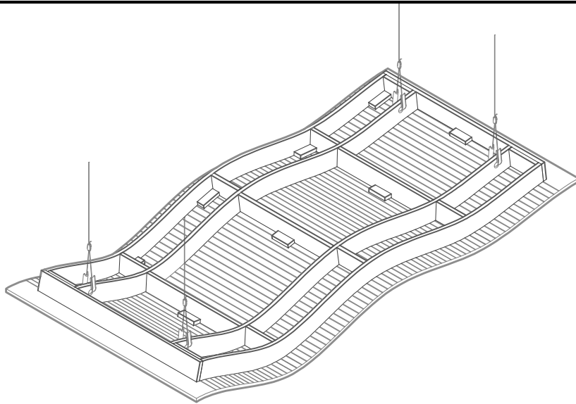
ISOMETRIC
