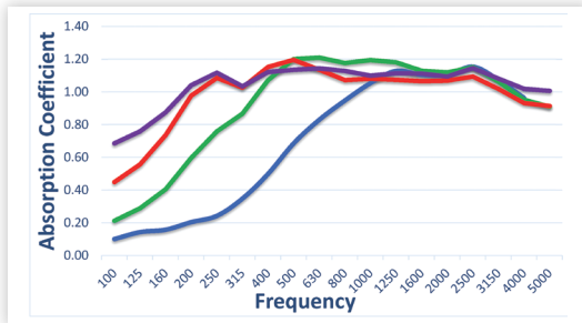
Blue = 1" Absorbor™ Panel = NRC 0.80, SAA 0.78 Green = 2" Absorbor™ Panel = NRC 1.00, SAA 1.06 Red = 3" Absorbor™ Panel = NRC 1.00, SAA 01.09 Purple = 4" Absorbor™ Panel = NRC 1.00, SAA 1.10
