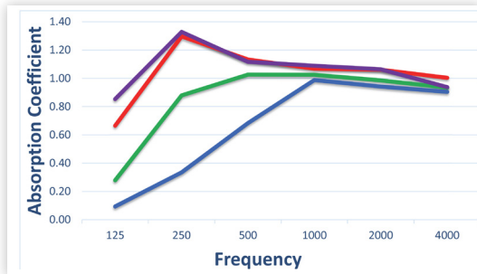
Blue = 1" Ultra Hi-Impact Absorbor Panel™ = NRC 0.75 Green = 2-1/8" Ultra Hi-Impact Absorbor Panel™ = NRC 1.00 Red = 3" Ultra Hi-Impact Absorbor Panel™ = NRC 1.00+ Purple = 4" Ultra Hi-Impact Absorbor Panel™ = NRC 1.00+
