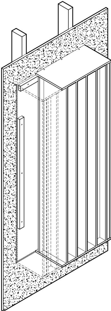
SECTIONAL ISOMETRIC VIEW SHOWING CLEAT LOCATION
