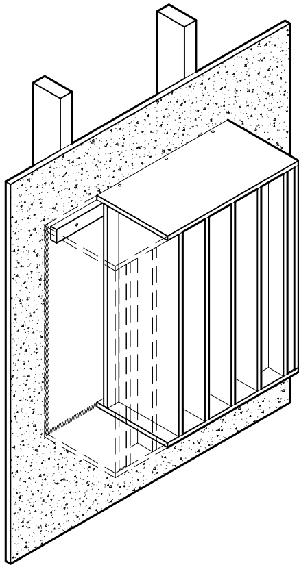
SECTIONAL ISOMETRIC VIEW SHOWING CLEAT LOCATION
