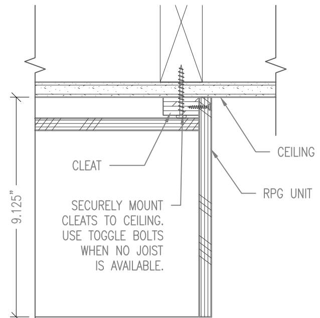
SECTION AT CLEAT
