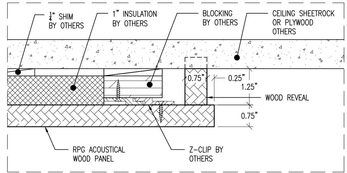
B-DETAIL SECTION
