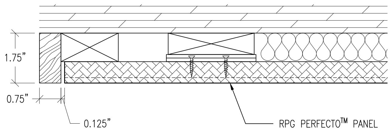
A-DETAIL SECTION @ TRIM
