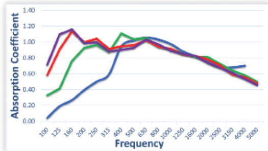
Blue = 1" 6lb/ft 3 fiberglass board Green = 2" 6lb/ft 3 fiberglass board Red = 3" 6lb/ft 3 fiberglass board Purple = 4" 6lb/ft 3 fiberglass board
