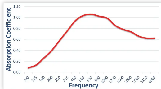
The sound absorption chart above represents the average Dado™ Absorptive Wood Panel or Plank acoustical performance based on the 3mm groove width at the face of the panel. Several factors play into the exact performance, such as cavity depth and contents of the cavity. Precise data for project requirements can be provided upon request.
