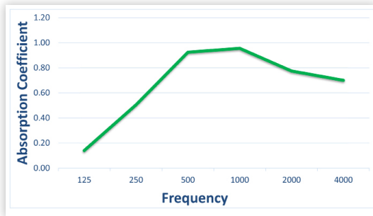
Green = Dado Panel + 1" 6lb/ft 3 fiberglass board
