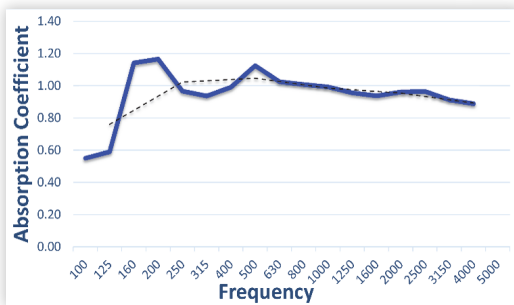
Blue = 16/16/8 Perfecto® on 6lb/ft 3 Fiberglass Board - NRC=1.00
