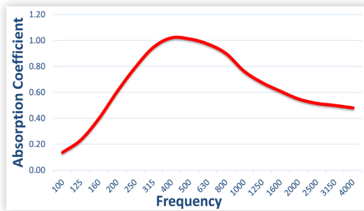
Red = 1" 6lb/ft 3 Fiberglass Board (predicted)
