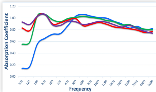
Blue = 1" 6lb/ft 3 Fiberglass Board (predicted) Green = 2" 6lb/ft 3 Fiberglass Board (predicted) Red = 3" 6lb/ft 3 Fiberglass Board (predicted) Purple = 4" 6lb/ft 3 Fiberglass Board (predicted)
