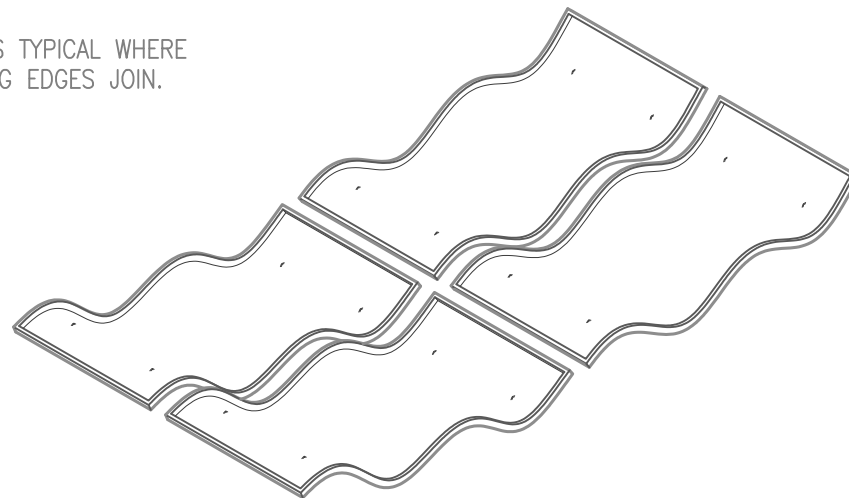
SPLINE ARRAY (EXPLODED)
