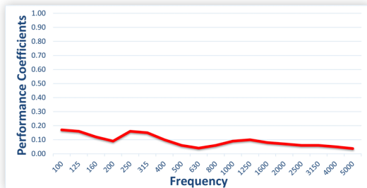
Red = Absorption Coefficient - NRC = 0.10
