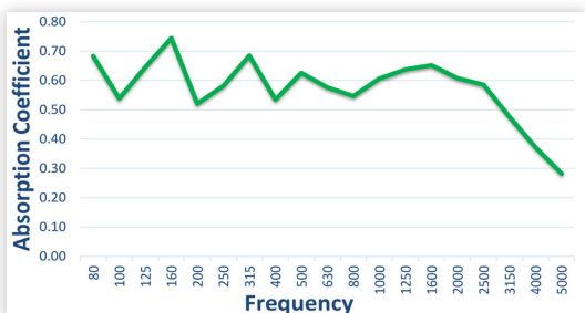
Green = Dual Layer Clearsorber® Foil System, 1-1/2" airspace between layers, 16" airspace behind System to substrate - NRC=0.60, SAA=0.60
